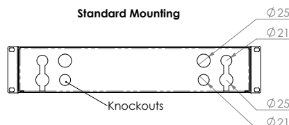
Standard Mounting
