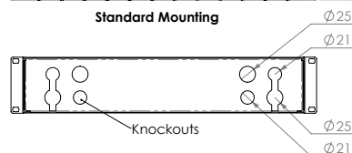
Standard Mounting
