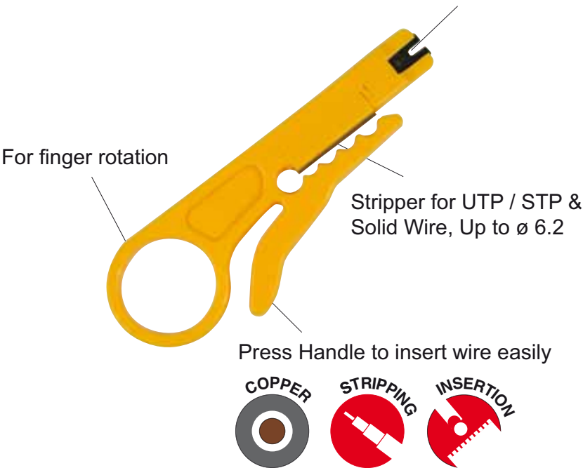
Economic Insertion Tool for use on 110 / 88 Type (Steel)
